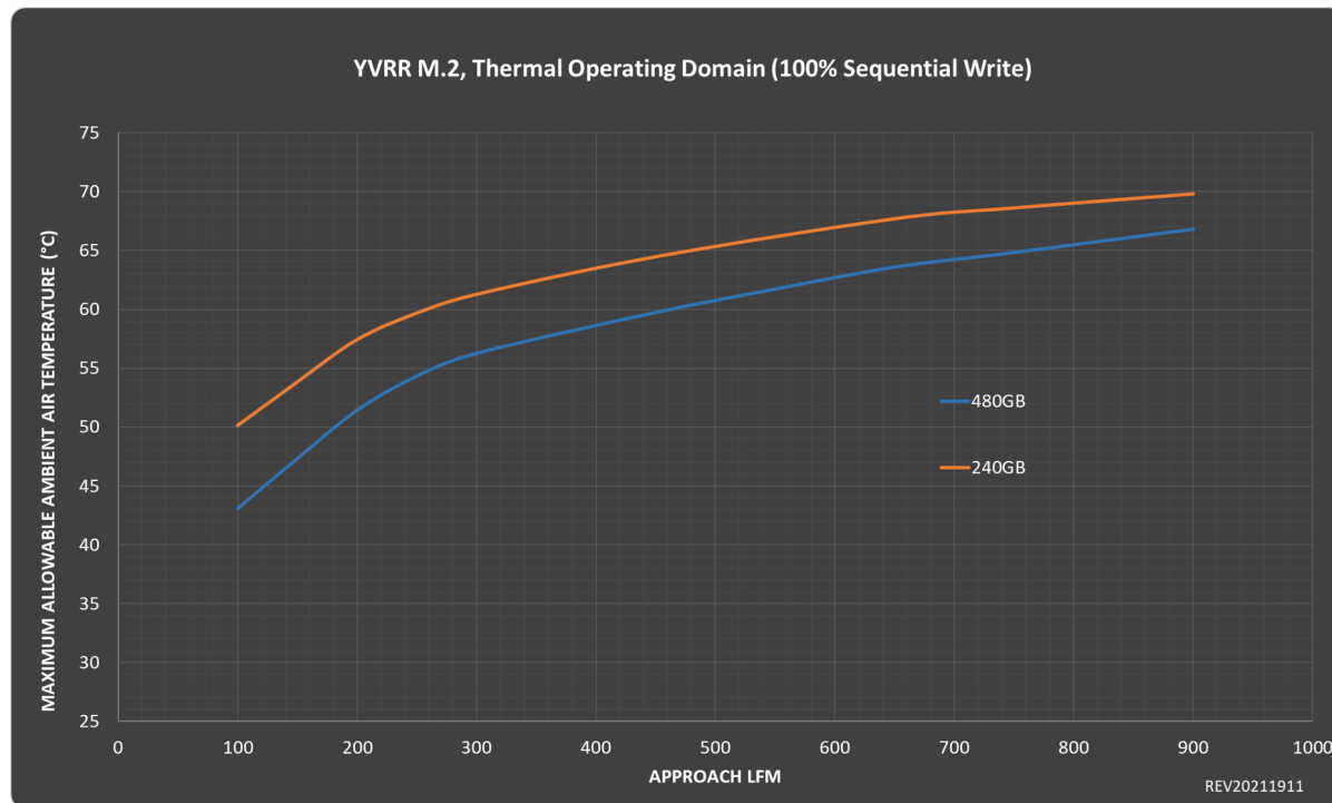
Figure 4: D3-S4520 Series Operating Domain Curves (M.2)
